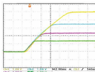
Power-Up Tracking
