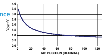
THE ISL85001 V OUT vs THE ISL22317W TAP POSITION
