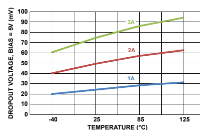
Ultra Low Dropout vs Temp vs Load
