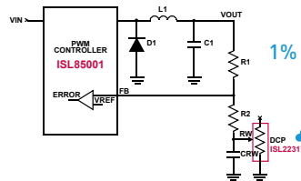
ADJUSTABLE POINT OF LOAD DC/DC REGULATOR
