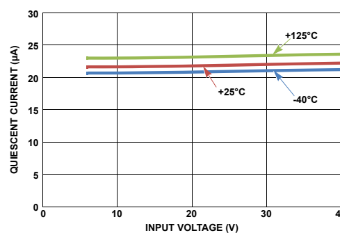
Quiescent Current vs Input Voltage (No Load)
