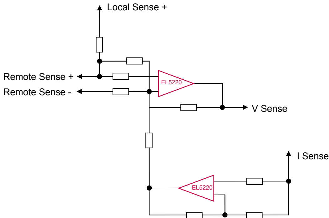
Typical OVP/OCF Application Circuit
