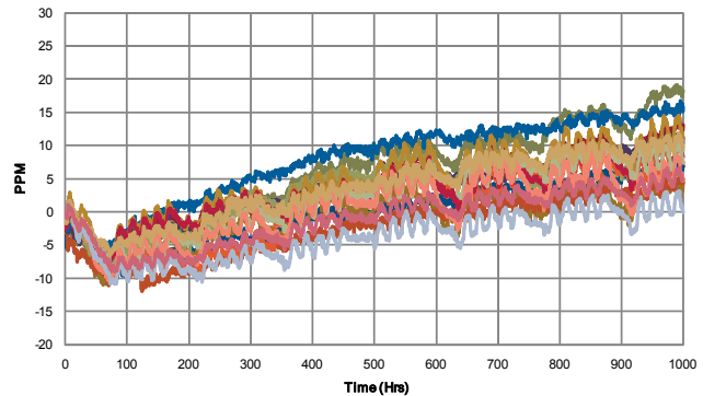
ISL21090 Long Term Drift Data (1000 Hrs)
