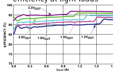
EFFICIENCY vs LOAD (1MHz 5VIN PFM)
